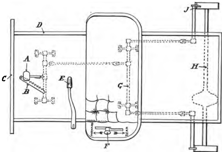
FIG. 301.—Diagram of the Controlling Apparatus of a Columbia Light Electric Vehicle. A, brake pedal; B, ratchet retaining pedal in place, operated by left foot; C, dash board; D, body sill; E, steering handle; F, controller handle; G, rocker shaft for setting hub brakes; J, brake band on wheel hub; H, rear axle.
